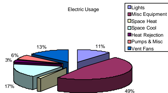
Figure 4: Shedd Electric Usage Profile
