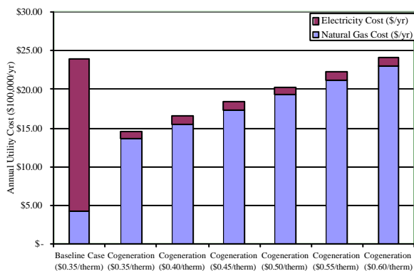
Figure 9: Annual Operating Cost Comparison
